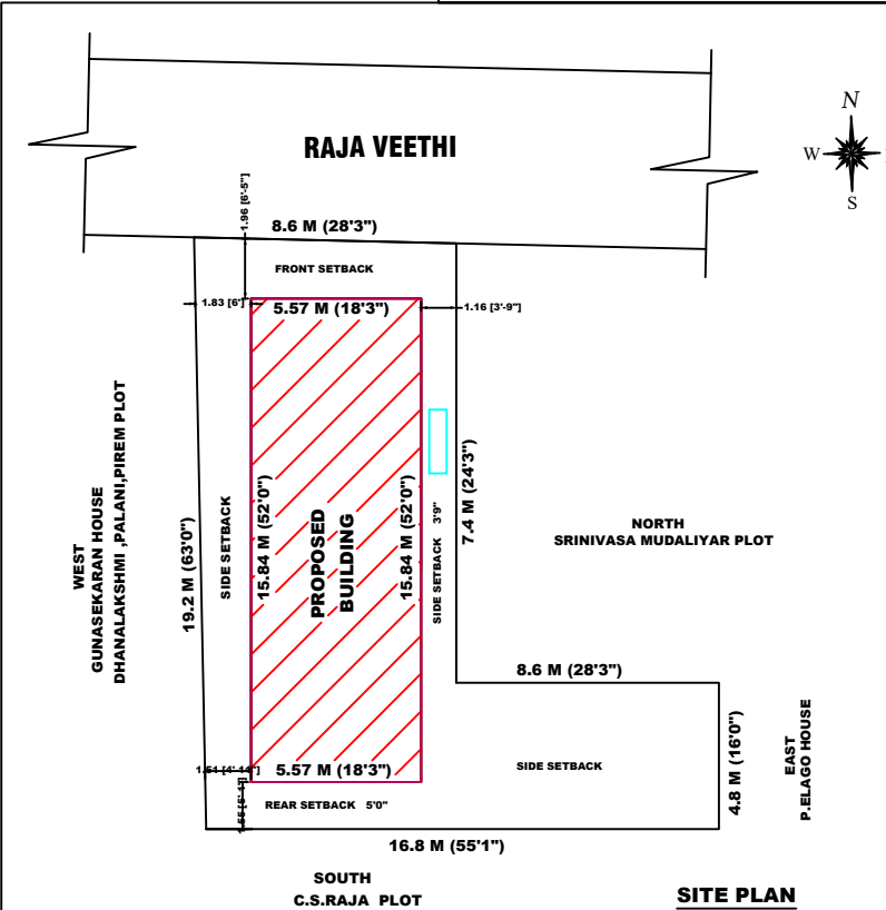
SITE PLAN
