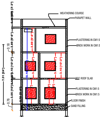
SECTION - AB'
