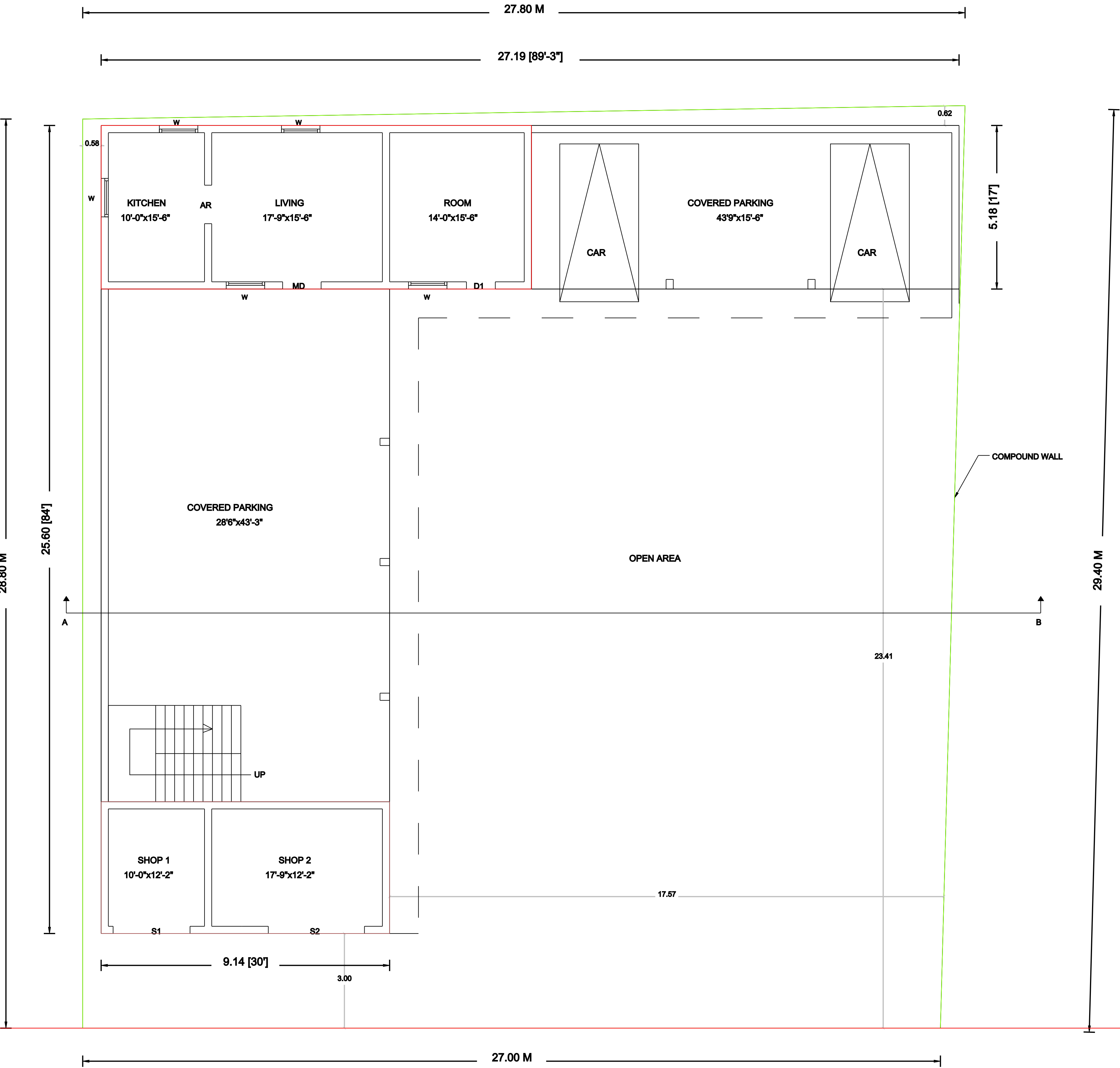
SITE CUM GROUND FLOOR PLAN
