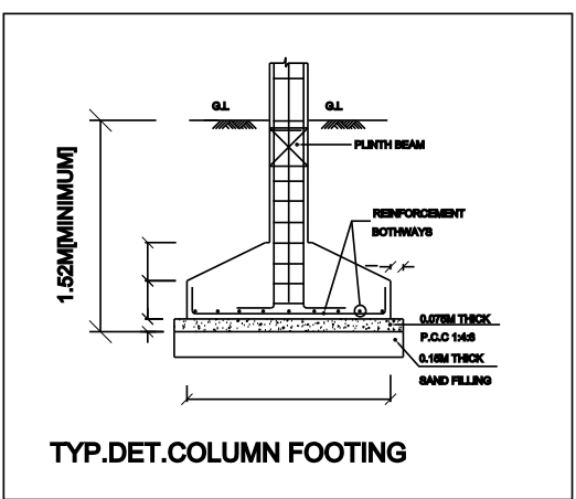
TYP.DET.COLUMN FOOTING
