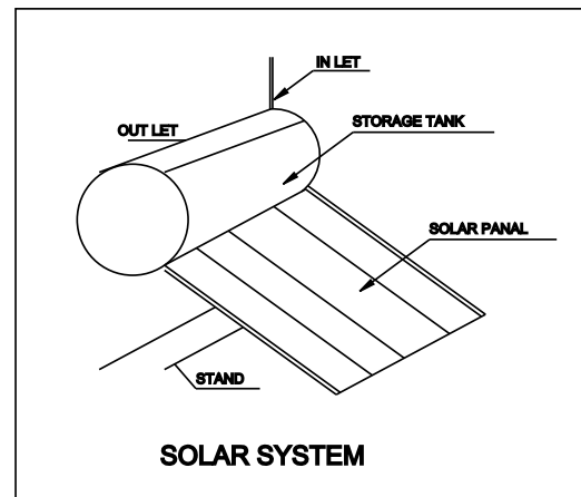
SOLAR SYSTEM
