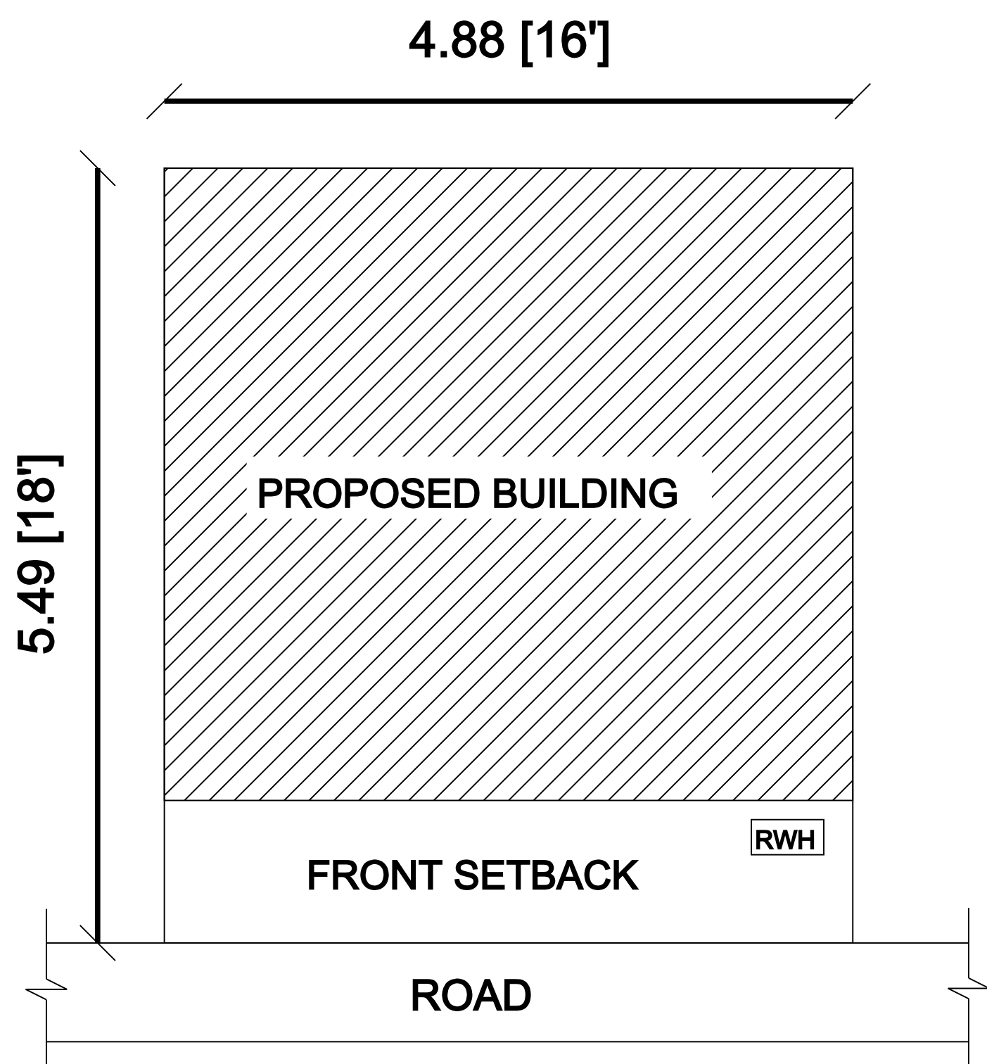
SITE PLAN
