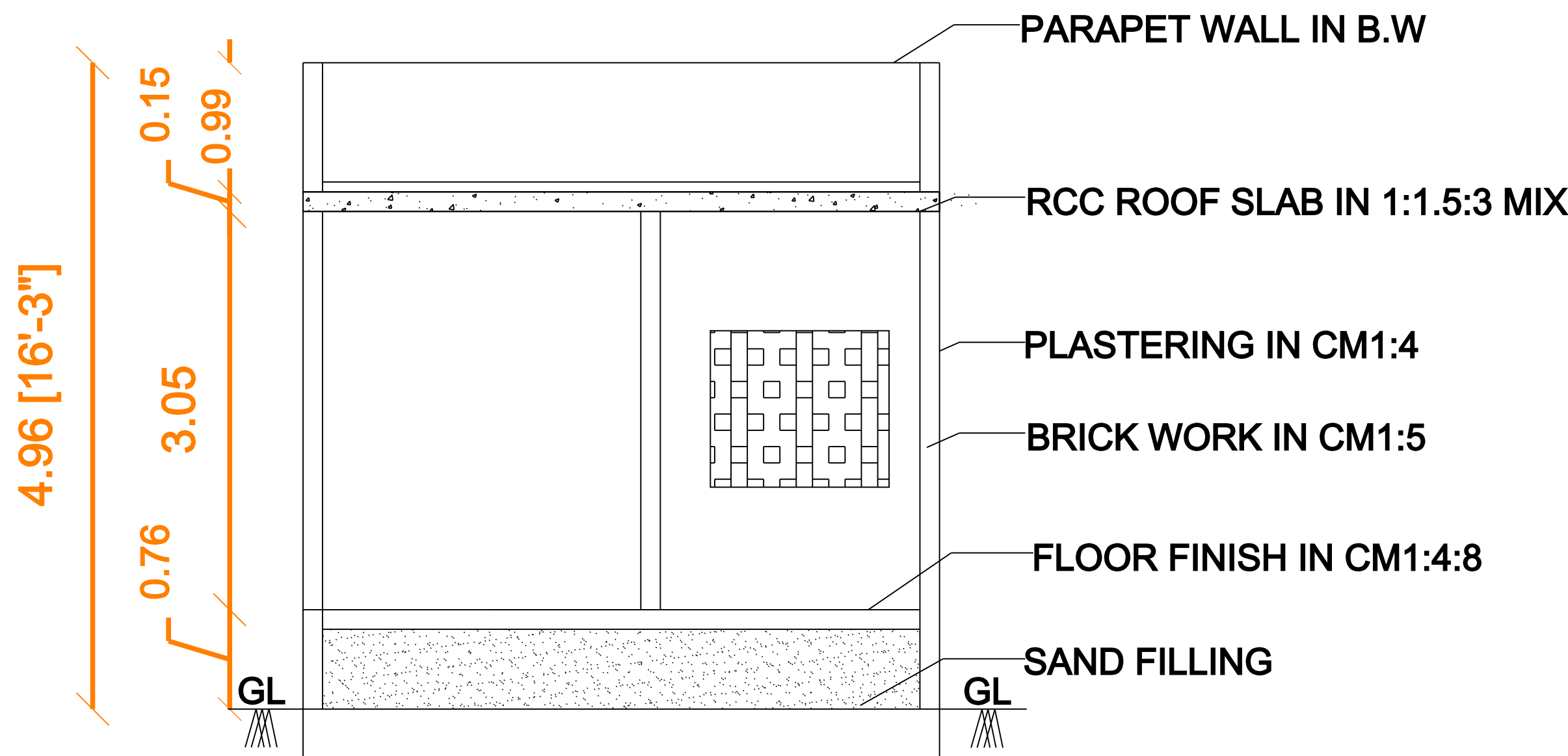
SECTION - AB'
