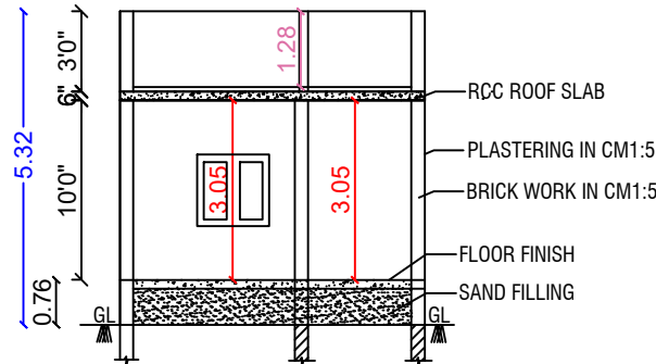
SECTION - AB'
