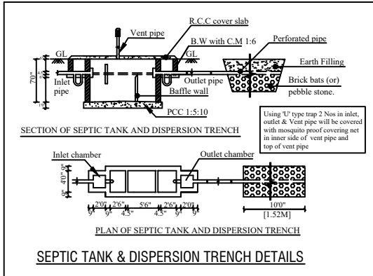
SEPTIC TANK & DISPERSION TRENCH DETAILS
