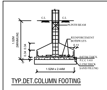
TYP.DET.COLUMN FOOTING
