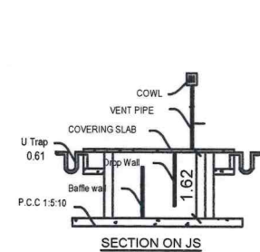
SECTION ON JS
