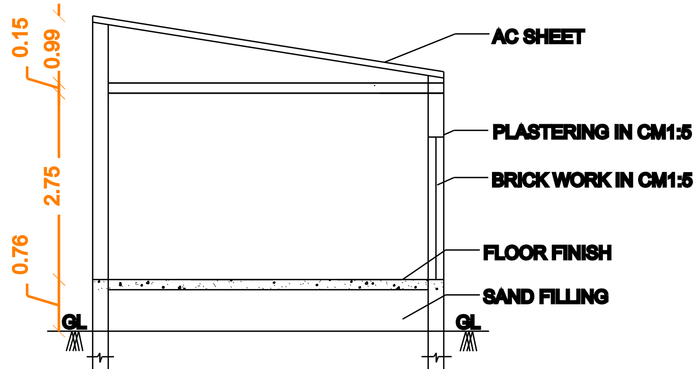
SECTION - AB'
