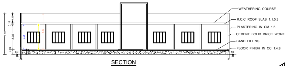
SECTION
