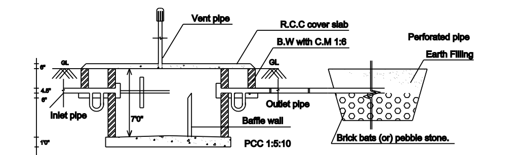
SECTION OF SEPTIC TANK AND DISPERSION TRENCH
