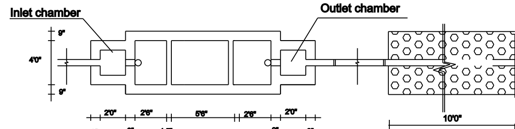
PLAN OF SEPTIC TANK AND DISPERSION TRENCH
