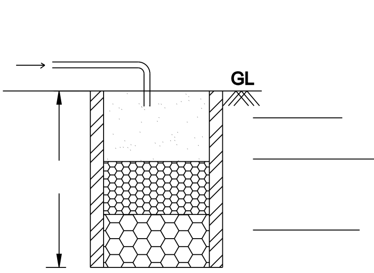
SECTION ON RAIN WATER COLLECTION TANK
