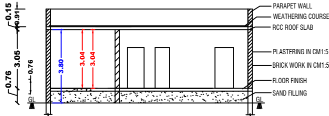
SECTION - AB'
