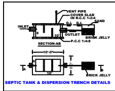
SEPTIC TANK & DISPERSION TRENCH DETAILS
