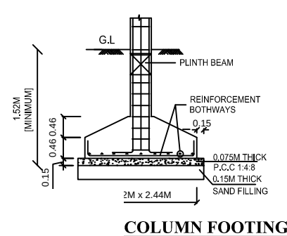
COLUMN FOOTING
