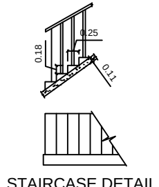
STAIRCASE DETAIL
