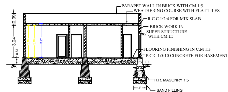
SECTION ON 'RS'
