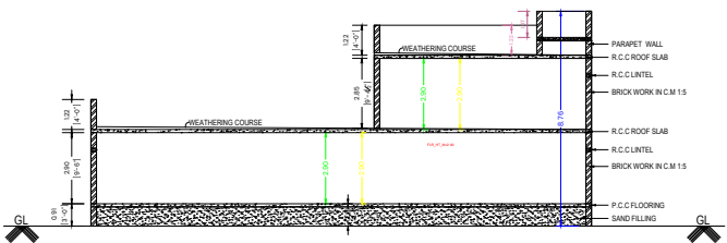
SECTION VIEW L-L
