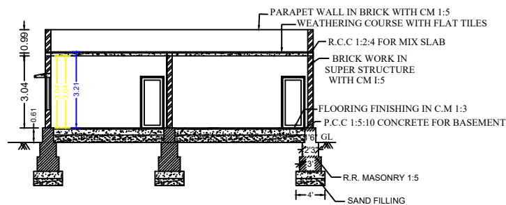
SECTION ON 'RS'
