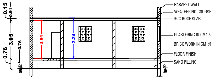
SECTION - AB'
