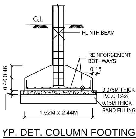
YP. DET. COLUMN FOOTING
