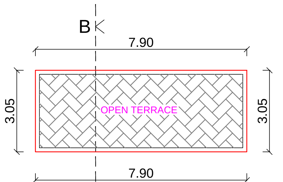
TERRACE PLAN
