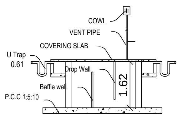
SECTION ON JS
