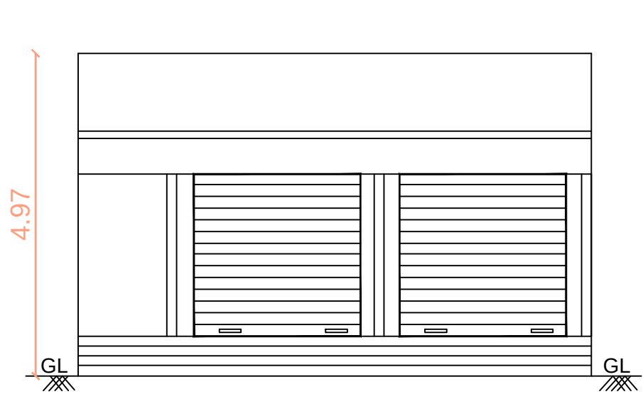
FRONT ELEVATION
