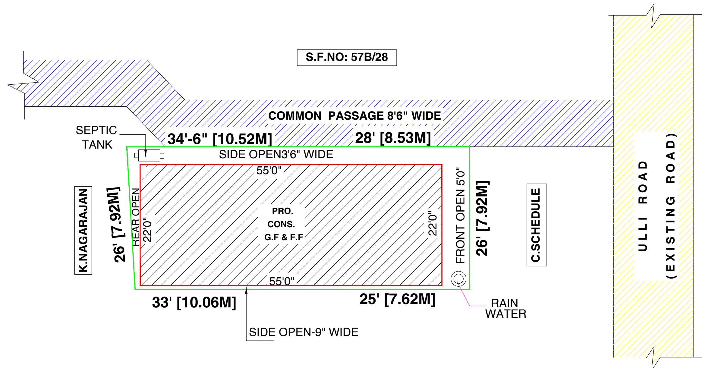
SITE PLAN SCALE - 1CM = 2M
