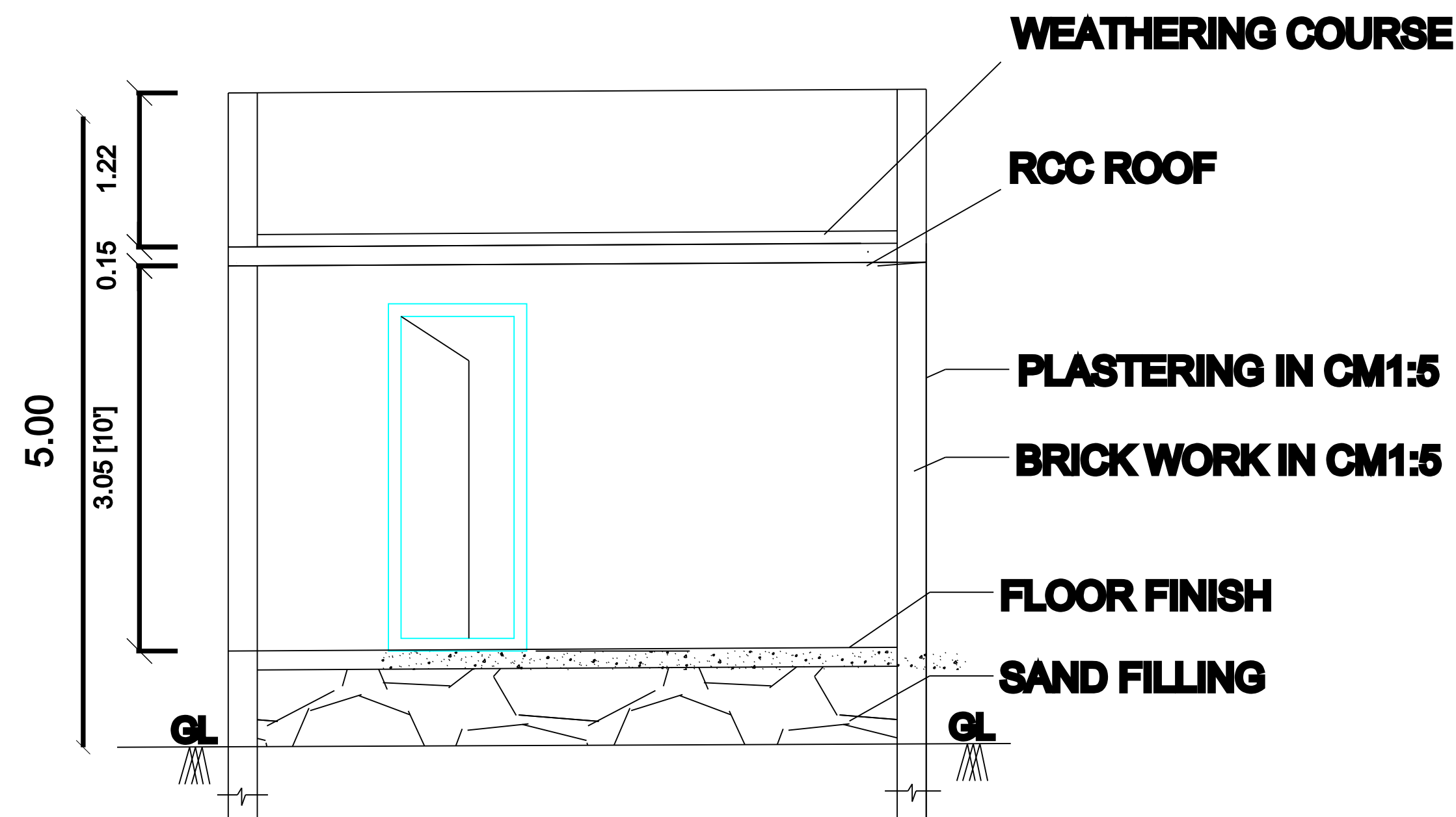
SECTION - AB'
