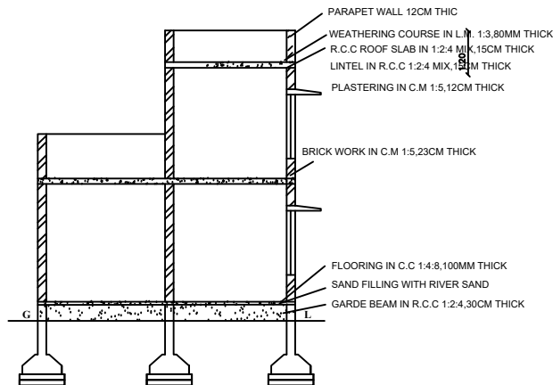
SECTION
