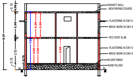
SECTION - AB'
