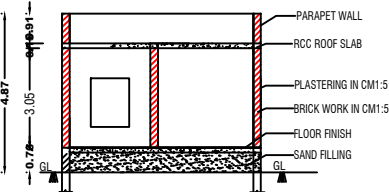
SECTION - AB'
