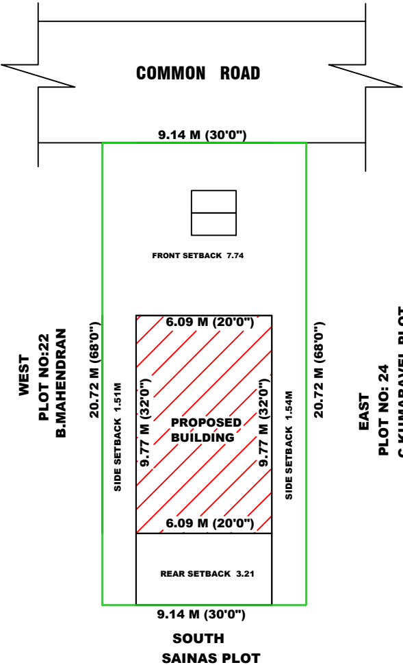
SITE PLAN
