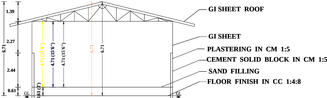
SECTION
