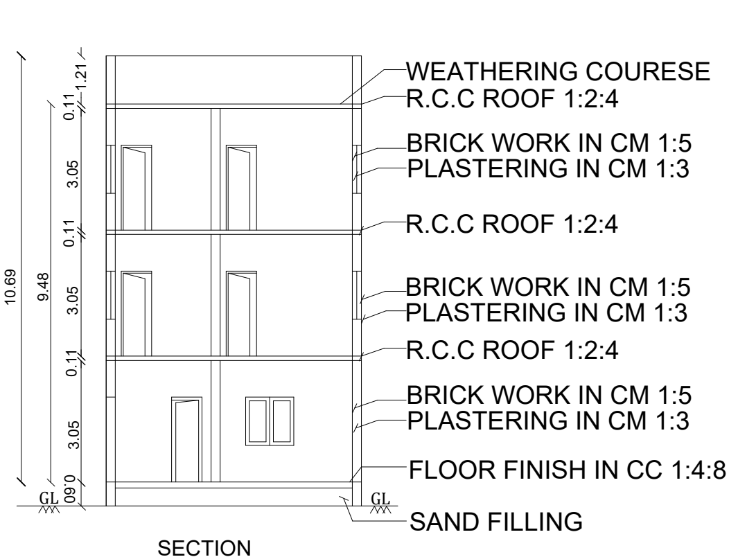
SECTION
