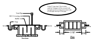
SEPTIC TANK WITH U TRAP
