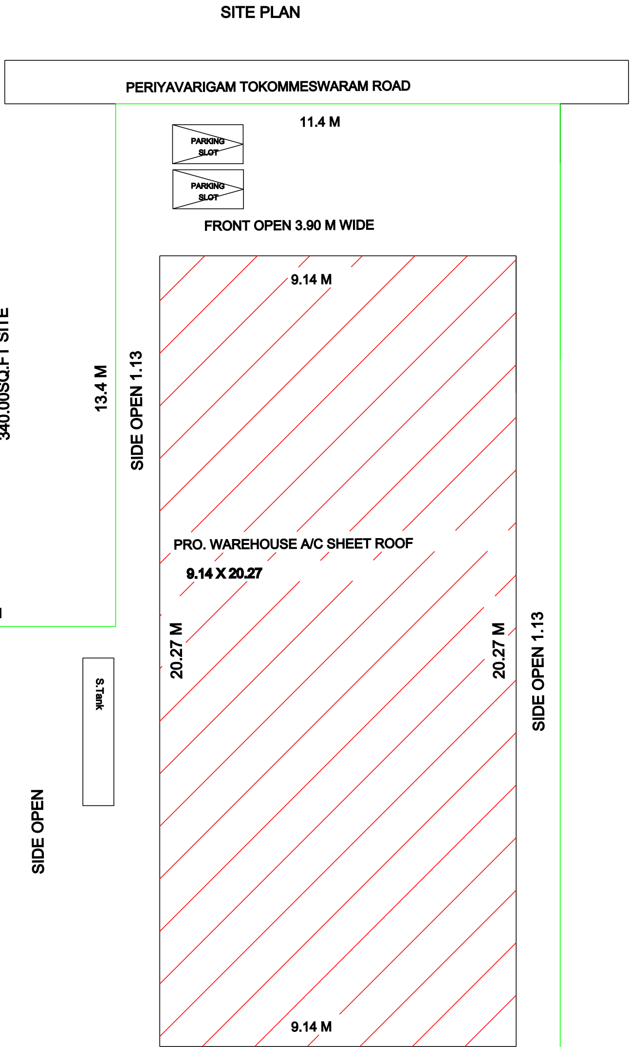
SITE PLAN
