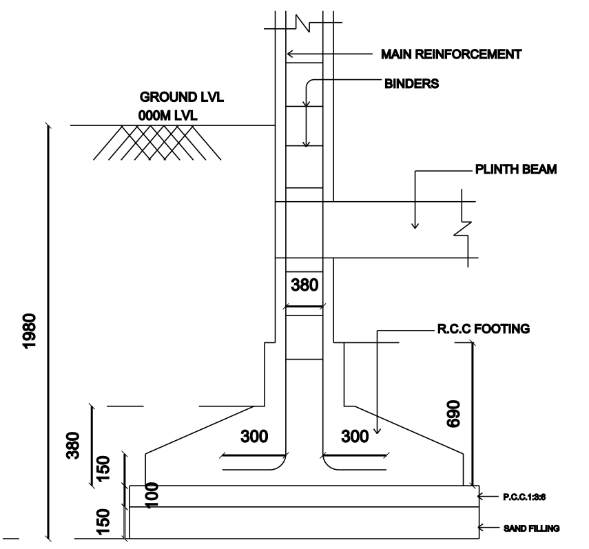
TYPICAL SECTION OF R.C.C COLUMN FOUNDATION
