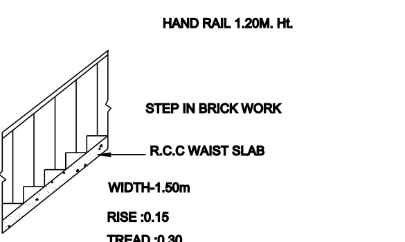
HAND RAIL 1.20M, H.L.
