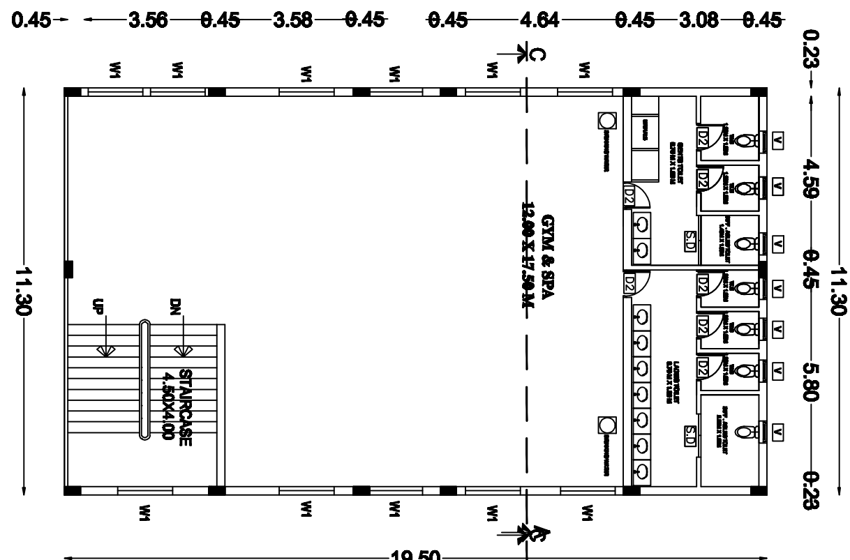
FIRST FLOOR PLAN BLOCK-10 GYM & SPA
