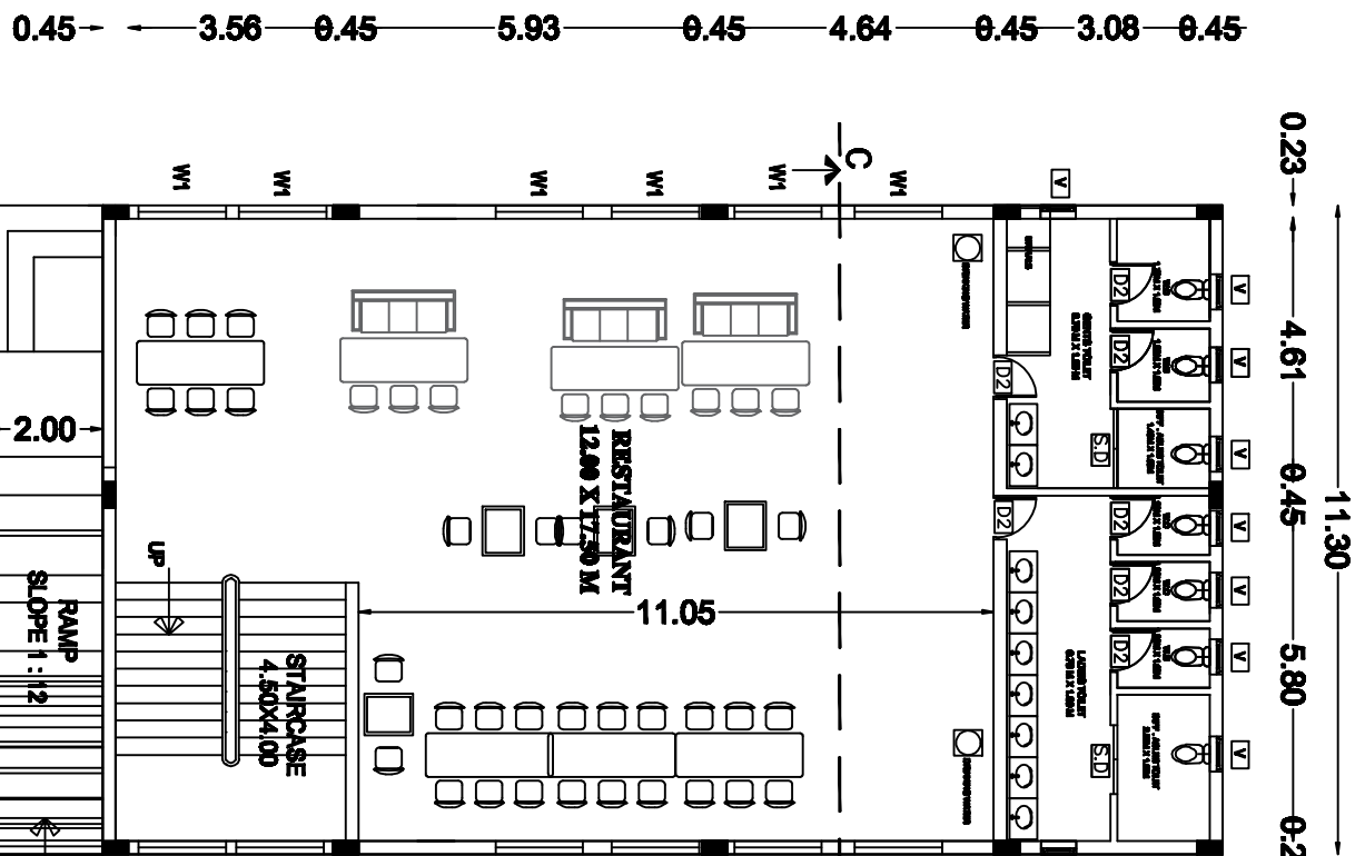
GROUND FLOOR PLAN BLOCK-10 HOTEL / RESTAURANT
