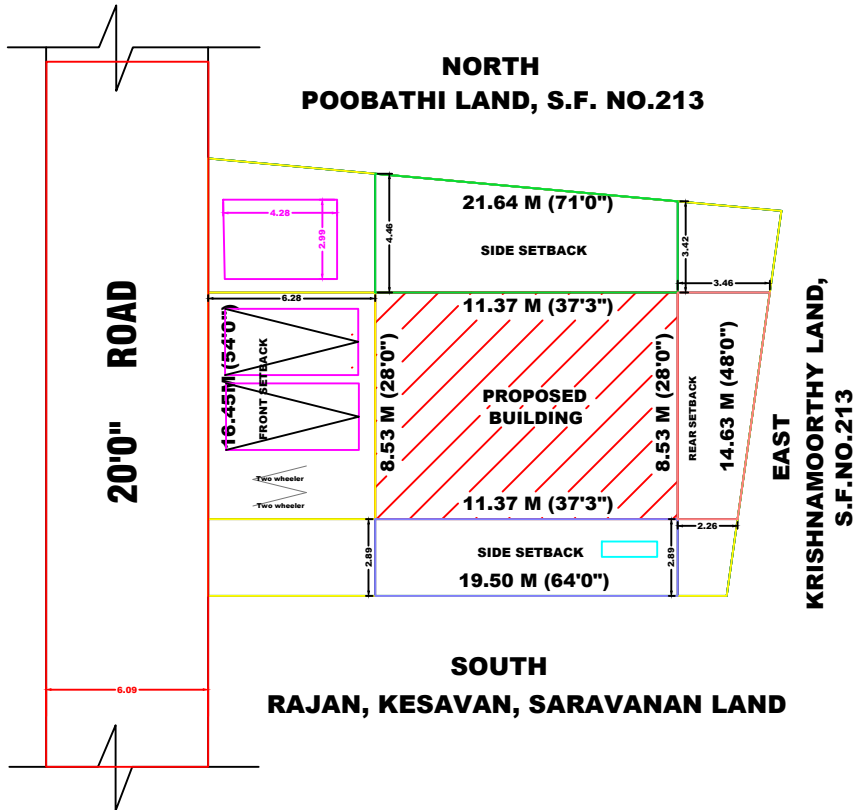
TOPO PLAN
