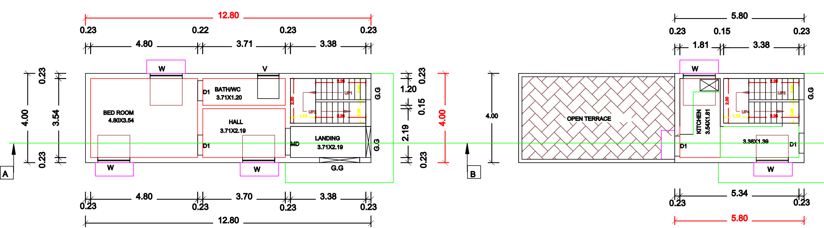
FLOOR-FIRST
