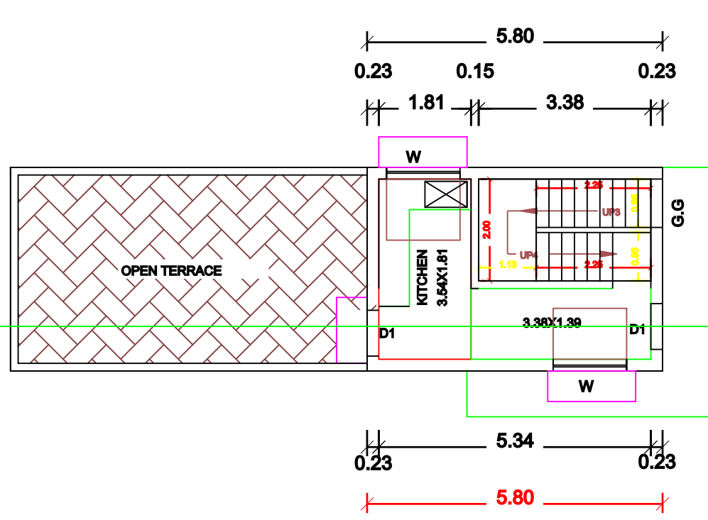
FLOOR-FIRST
