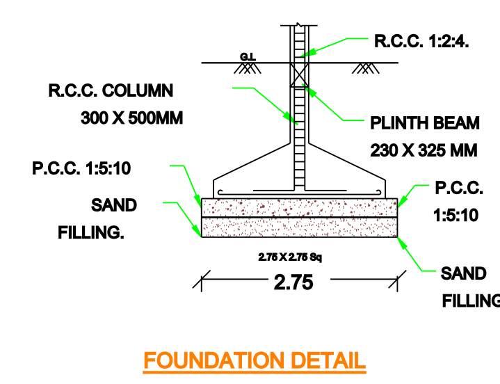
FOUNDATION DETAIL
