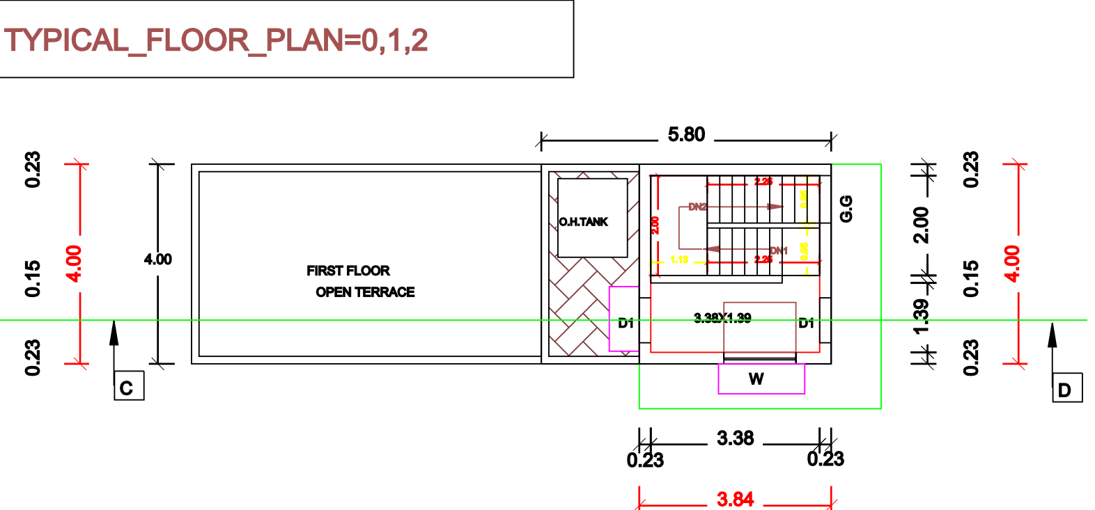
FLOOR-SECOND
