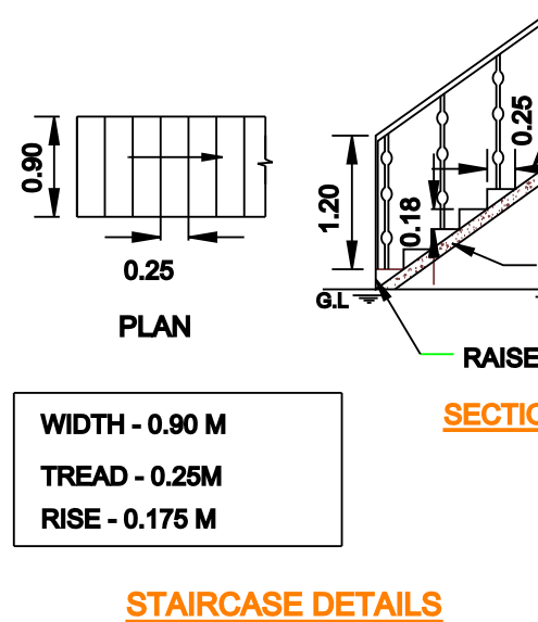
STAIRCASE DETAILS
