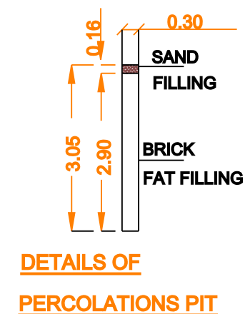
DETAILS OF PERCOLATIONS PIT
