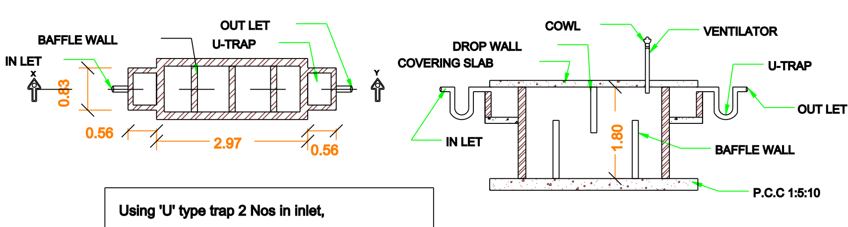
SECTION ON 'XY'
