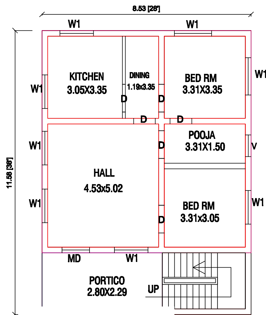
PLAN
