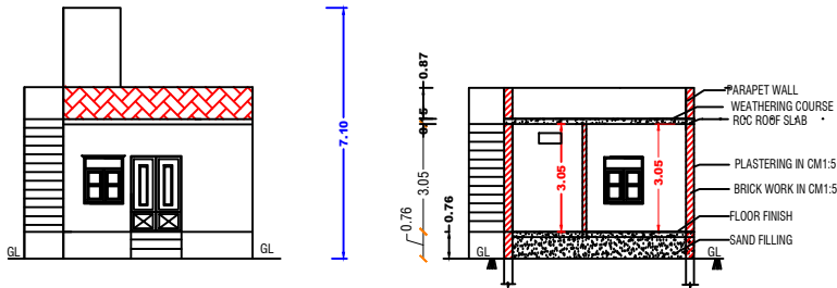
SECTION - AB'
