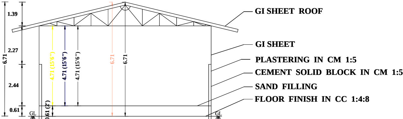
SECTION
