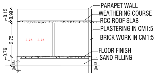
SECTION - AB'
