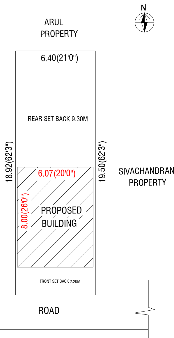
SITE PLAN
