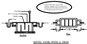
SEPTIC TANK WITH U TRAP
