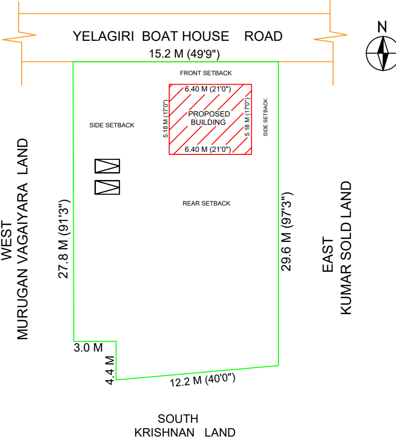
SITE PLAN
