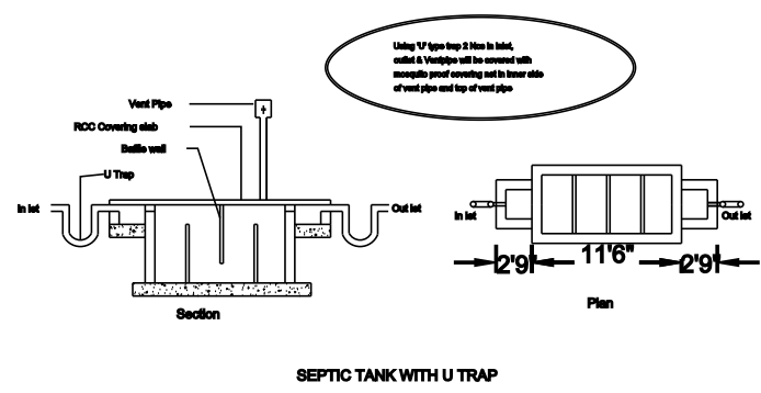
SEPTIC TANK WITH U TRAP
