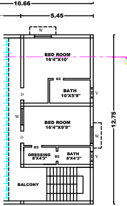
F FLOOR PLAN
