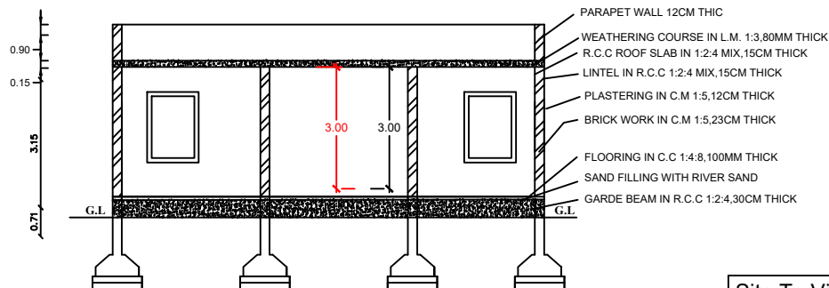
SECTION
