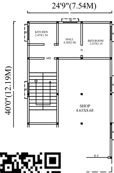
GR PLAN
