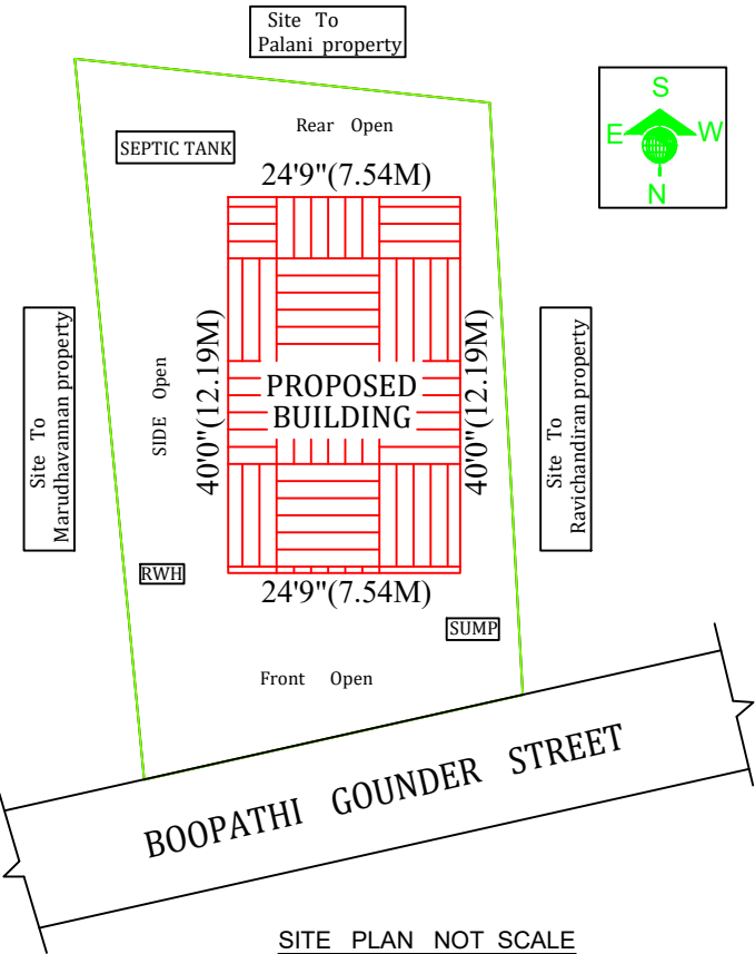
SITE PLAN NOT SCALE
