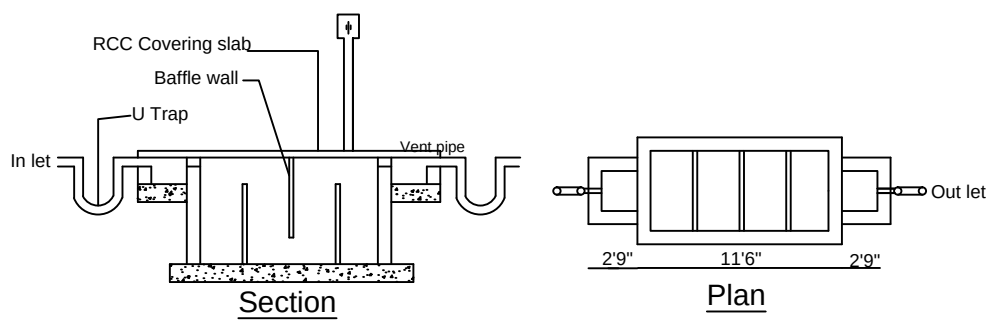
Septic tank with U Trap
