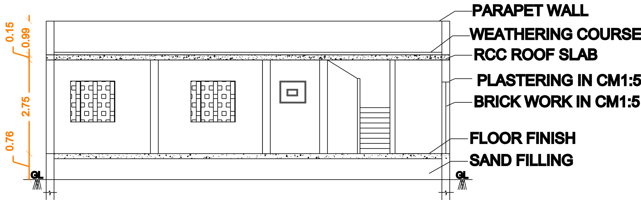
SECTION - AB'
