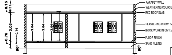
SECTION - AB'
