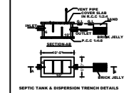
SEPTIC TANK & DISPERSION TRENCH DETAILS
