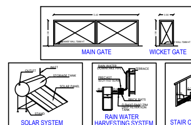
RAIN WATER HARVESTING SYSTEM
