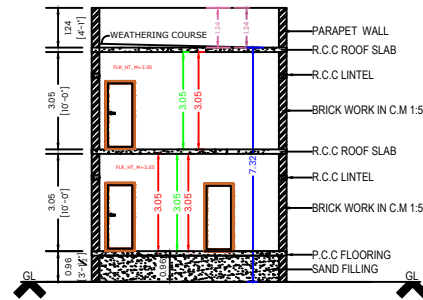
SECTION VIEW L-L
