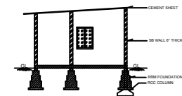
SECTION ON A-A FOR EXISTING BUILDING
