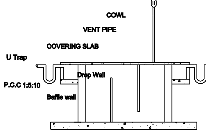
SECTION ON JS1
