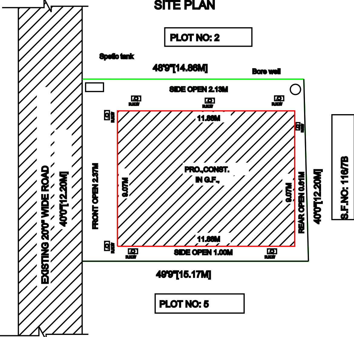
SITE PLAN DETAILS:-
