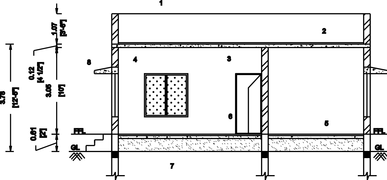
SECTION ON "JS"
