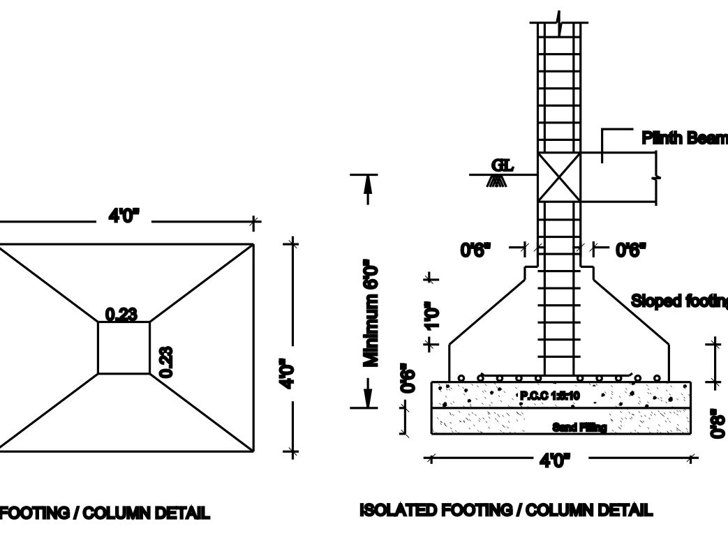
COLUMN DETAILS
