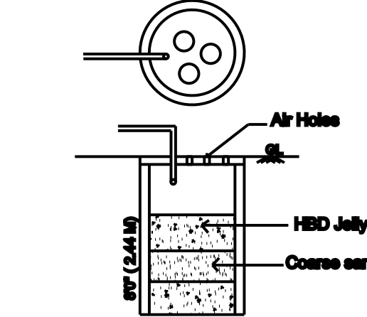
RAIN WATER HARVESTING TANK DETAIL
