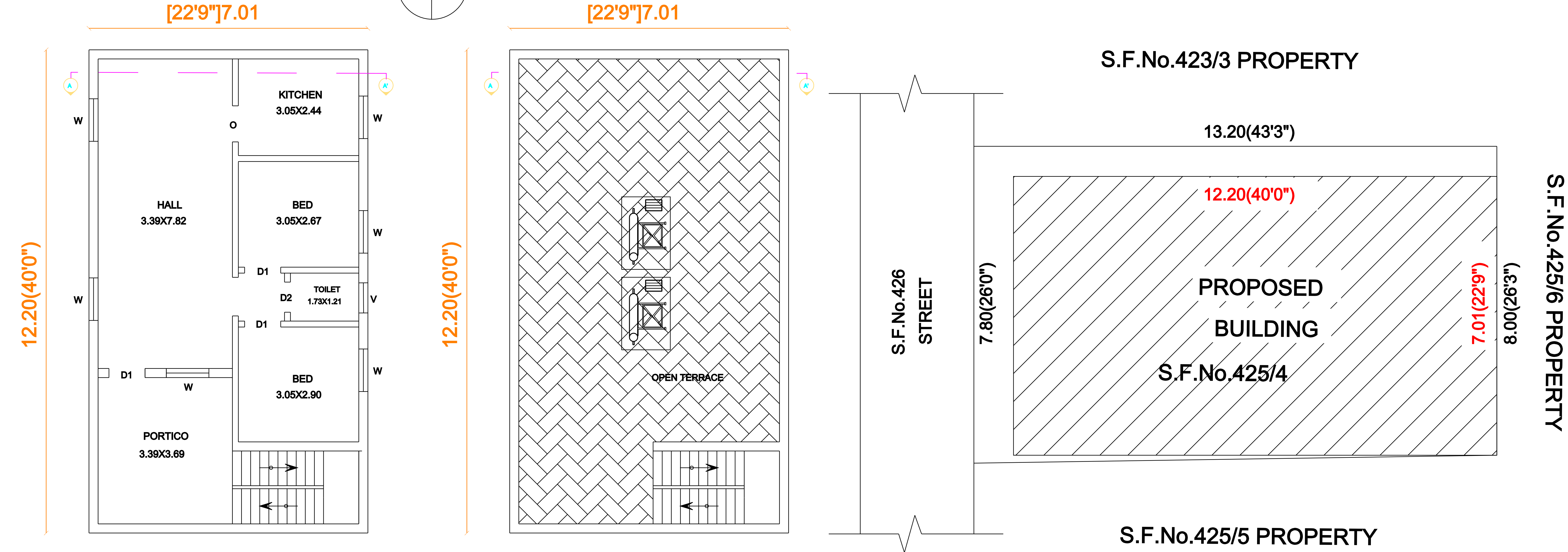
ND FLOOR PLAN
