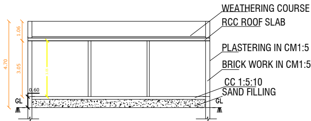
SECTION - AB'
