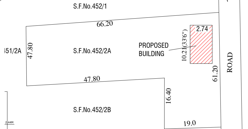
SITE PLAN
