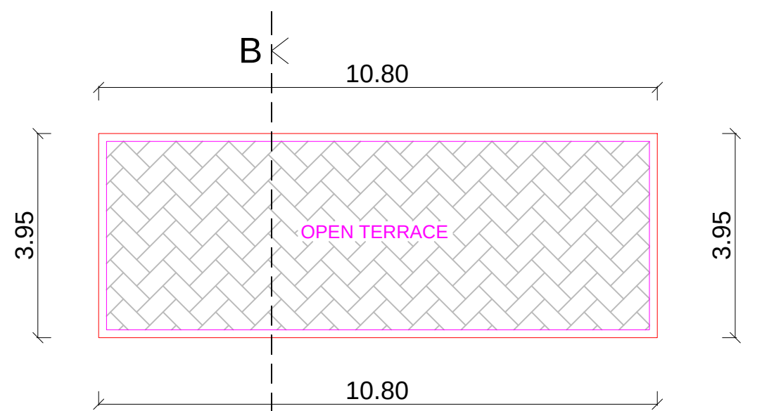
TERRACE PLAN
