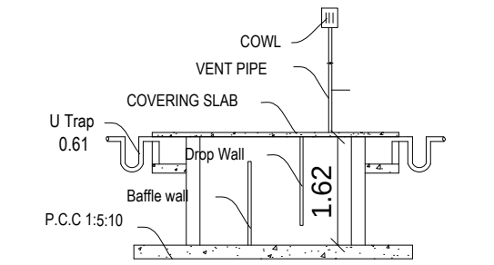
SECTION ON JS
