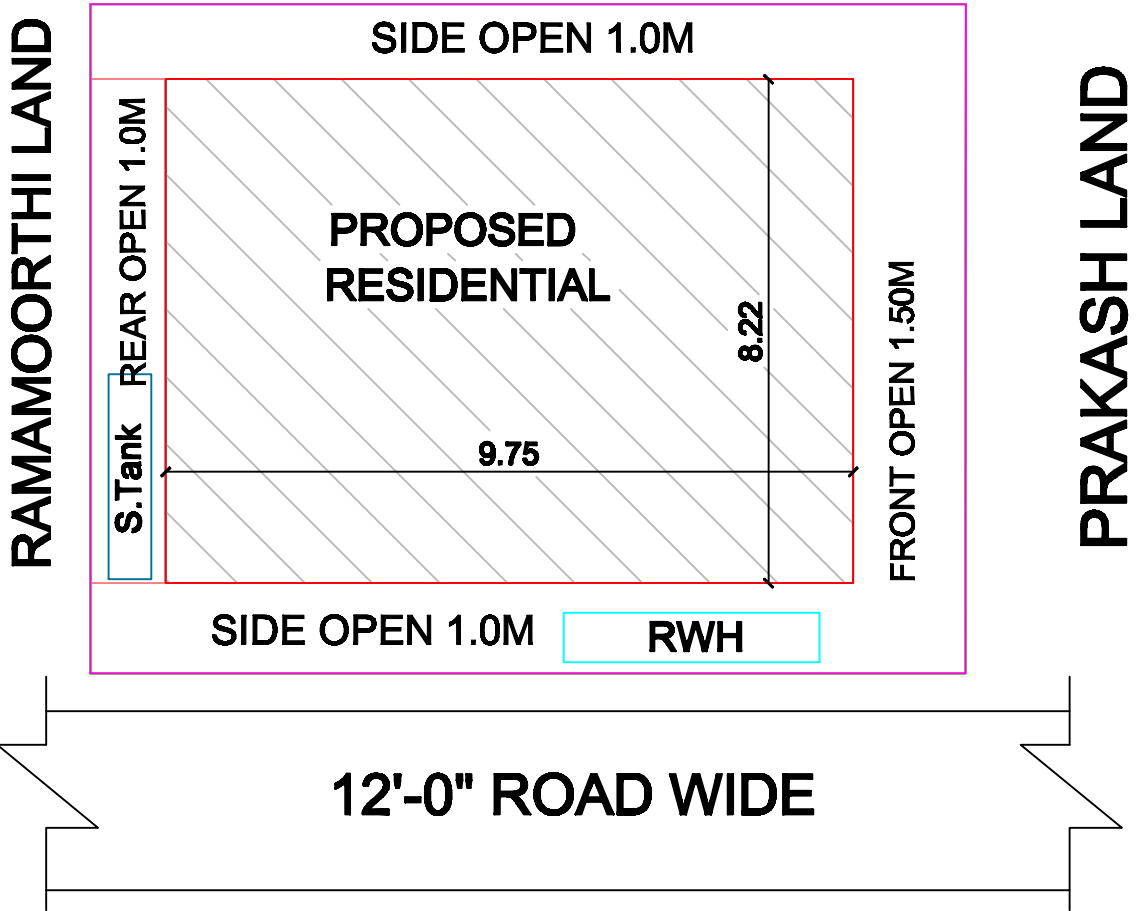
SITE PLAN
