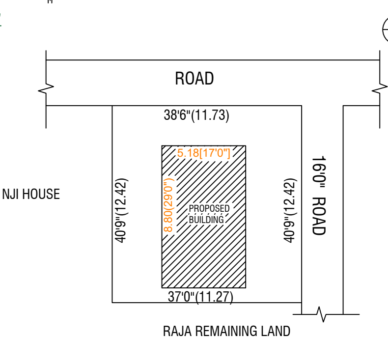
SITE PLAN
