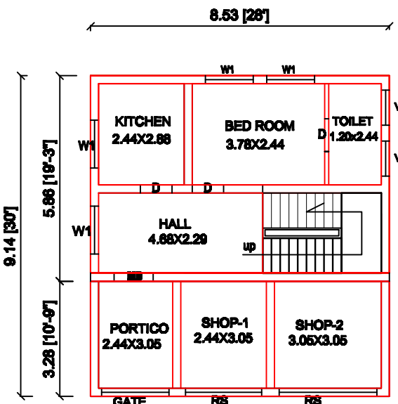
GROUND FLOOR PLAN COMMERCIAL & RESIDENTIAL
