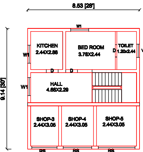
FIRST FLOOR PLAN COMMERCIAL & RESIDENTIAL
