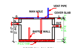
SECTION ON BB'
